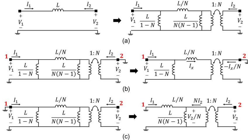
Fig. 2. (a) Norton transformation of a series floating inductor; (b) equivalent circuit for y_{11B} = I_1/V_1 and y_{21B} = I_2/V_1 ; (c) equivalent circuit for y_{12B} = I_1/V_2 and y_{22B} = I_2/V_2 .
