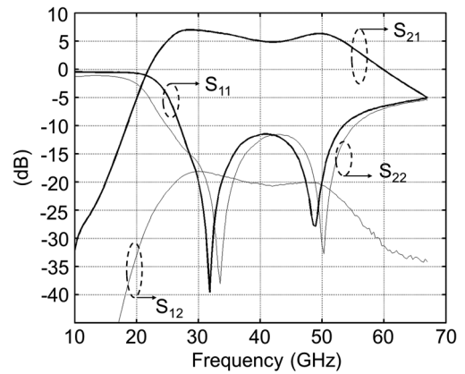
Fig. 7. BPDA measured S-parameters.
