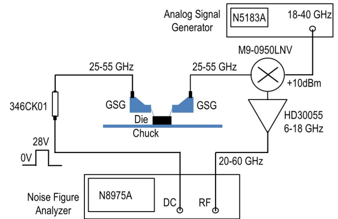
Fig. 8. Setup for BPDA noise characterization using the N8975A noise-figure analyzer.
