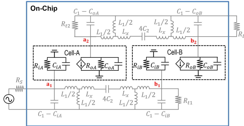
Fig. 4. Circuit diagram of the band-pass DA with representation of the input and output impedances associated with each gain-cell.
