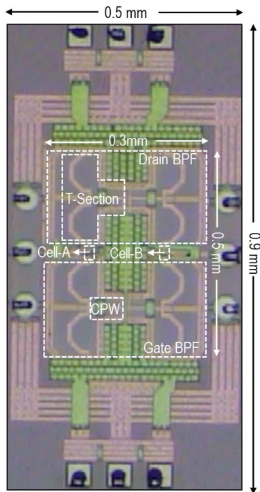
Fig. 6. Chip microphotograph for the BPDA.
