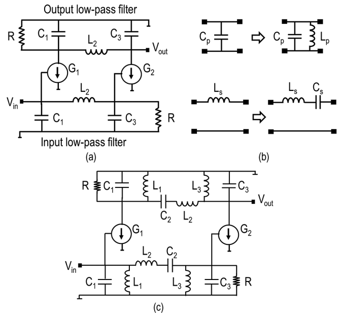
Fig. 1. (a) Canonical form of the LPDA (b) low-pass to band-pass filter transformation (c) canonical form of the BPDA.
