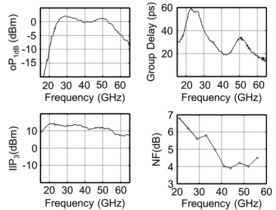
Fig. 9. Compression-point, group-delay, and IIP3 characterization versus frequency.
