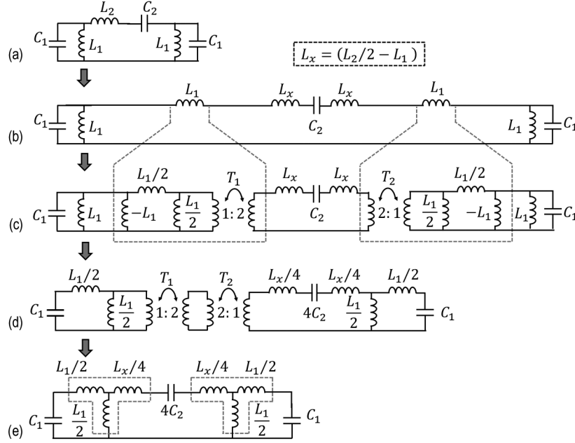
Fig. 3. Derivation of the compact-area bandpass filter starting with the canonical bandpass filter (top figure) through the application of mirror-symmetric dual Norton transforms.
